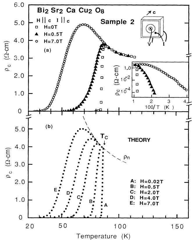
FIG. 2. (a) \rho_c for \mathbf{H} parallel to \mathbf{c} using the symmetric contact configuration shown schematically. Inset: Arrhenius plot of the same data. (b) Equation (4) (solid symbols) fitted to \rho_c(T < T_c) data in (a) with J_c(0) = 5.4 \times 10^{-6} A/cm 2 (see text). \rho_n fit by Eq. (2) is also shown.
