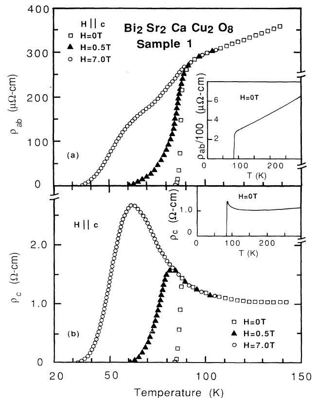
FIG. 1. (a) \rho_{ab} and (b) \rho_c vs T for \mathbf{H} parallel to c . The insets show zero-field behavior.
