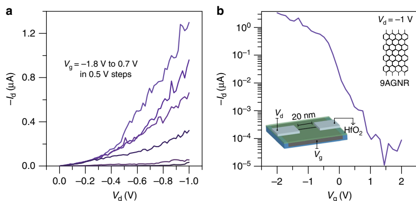
Fig. 5 Transport characteristics of a scaled, high-performance 9AGNRFET at room temperature. a I_d - V_d characteristics of the scaled 9AGNRFET. b I_d - V_g of the devices show high I_{\text{on}} > 1 \mu\text{A} for a 0.95 nm wide 9AGNR and high I_{\text{on}}/I_{\text{off}} \sim 10^5 . Inset : scaled 9AGNRFET schematic
