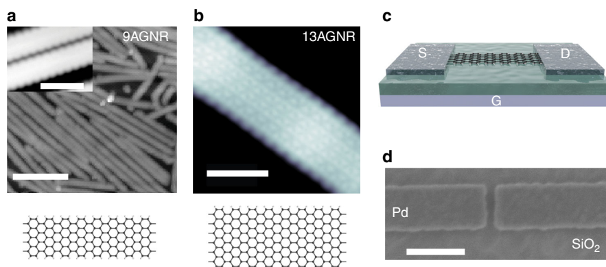
Fig. 1 High-resolution STM GNR characterization and FET structure. a STM image of synthesized 9AGNR on Au with a scale bar of 10 nm ( V_{\text{s}} = 1 \text{ V} , I_{\text{t}} = 0.3 \text{ nA} ). Inset: High-resolution STM image of 9AGNR on Au ( V_{\text{s}} = 1 \text{ V} , I_{\text{t}} = 0.5 \text{ nA} ) with a scale bar of 1 nm. b High-resolution STM image of 13AGNR on Au with a scale bar of 2 nm ( V_{\text{s}} = -0.7 \text{ V} , I_{\text{t}} = 7 \text{ nA} ). c Schematic of the short channel GNRFET with a 9AGNR channel and Pd source-drain electrodes. d Scanning electron micrograph of the fabricated Pd source-drain electrodes with a scale bar of 100 nm
