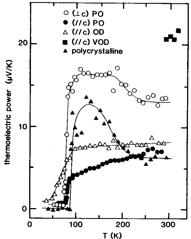
FIG. 2. Thermoelectric power (TEP) of single-crystal and polycrystalline \text{YBa}_2\text{Cu}_3\text{O}_y . Single-crystal TEP is shown for temperature gradients both perpendicular and parallel to the c axis. The c axis TEP is shown for three different oxygen contents. Solid lines are guides to the eye.
