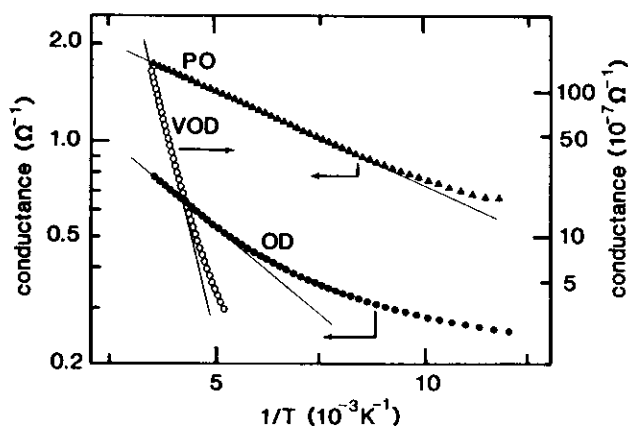
FIG. 3. Logarithm of conductivity vs 1/T shown for a single crystal along the c axis for three different oxygen contents. Linear regions indicate activated behavior. The activation energy increases with decreasing oxygen content.
