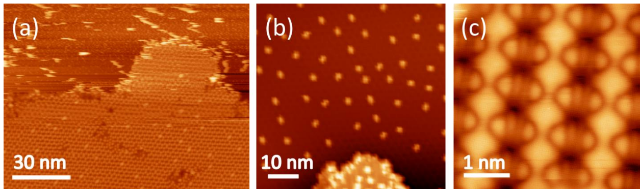
Figure S1: (a) A large scale STM image of F 4 TCNQ/graphene/BN at high molecular coverage ( V_s = 2 V, I_t = 10 pA, T = 4.5 K), (b) Single F 4 TCNQ molecules coexisting with a molecular island on graphene/BN ( V_s = 2 V, I_t = 5 pA, T = 4.5 K). (c) A zoom-in image of the island in (b) ( V_s = 2 V, I_t = 5 pA, T = 4.5 K).
